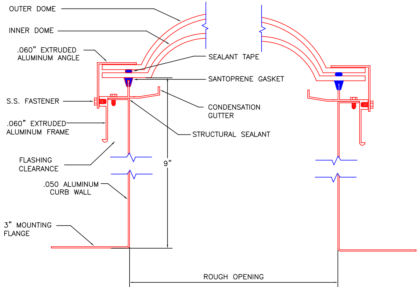
9" STANDARD SELF FLASHING (MODEL SF-9)
