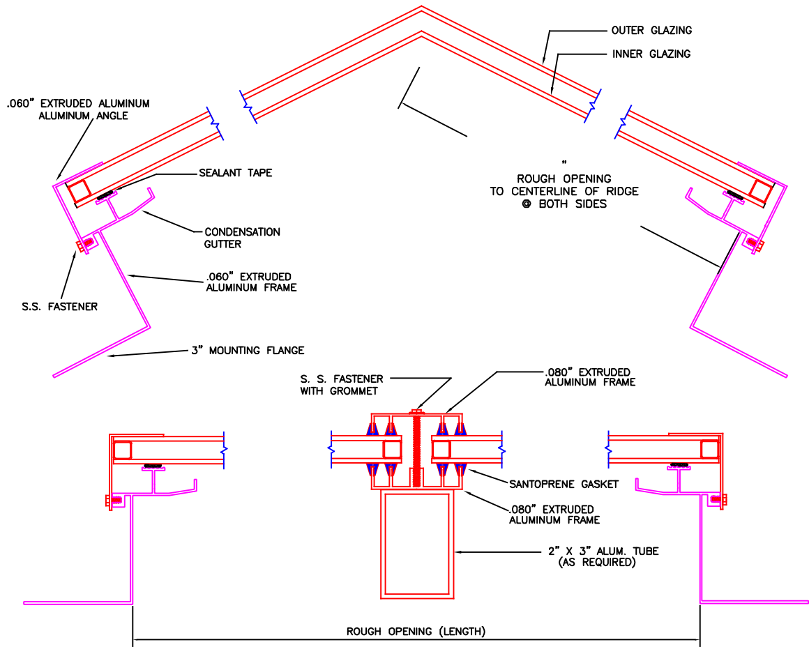
RIDGE MOUNT SELF FLASHING (MODEL RMSF)
