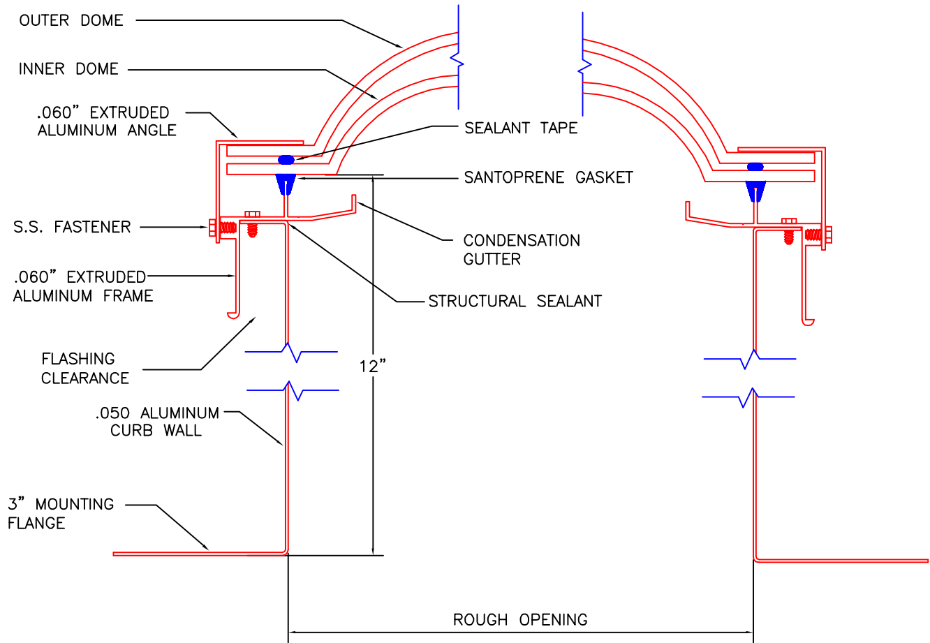
12" STANDARD SELF FLASHING (MODEL SF-12)
