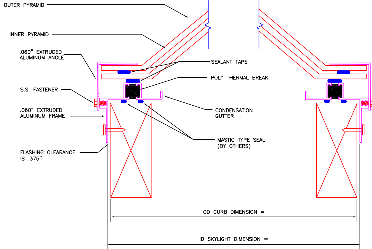
THERMALLY BROKEN CURB MOUNT – PYRAMID (MODEL TCM-PYR)
