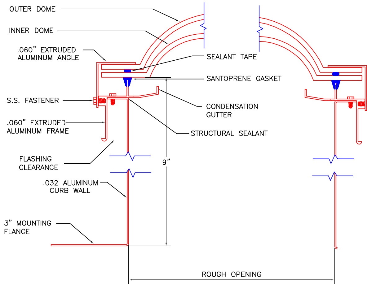
9" STANDARD SELF FLASHING (MODEL SF-9)
