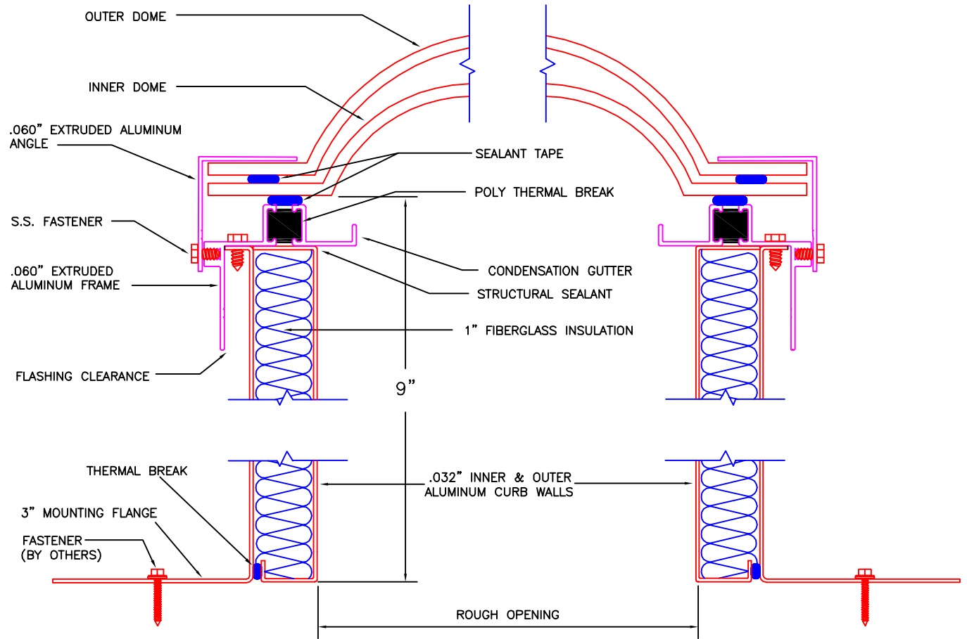
9" THERMALLY BROKEN & INSULATED SELF FLASHING (MODEL TSF-9)
